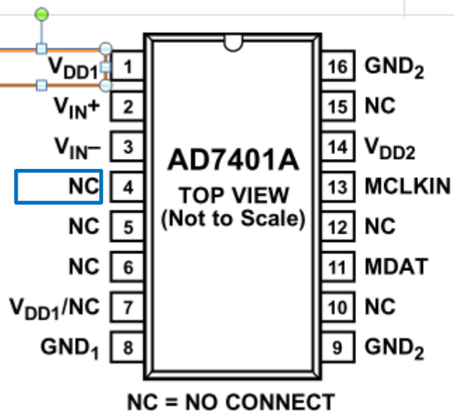
Figure 5. Pin Configuration
