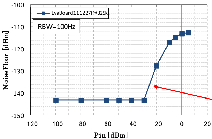
Noise Floor Measurement Result
