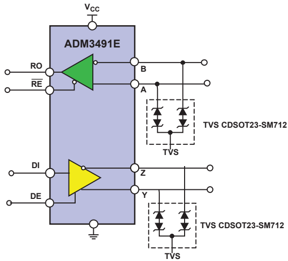
Protection Scheme 1—TVS
