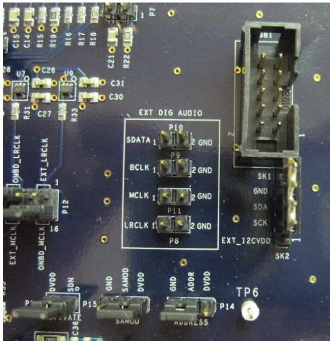
Figure 6: SSM2518 Stand Alone Mode Configuration
