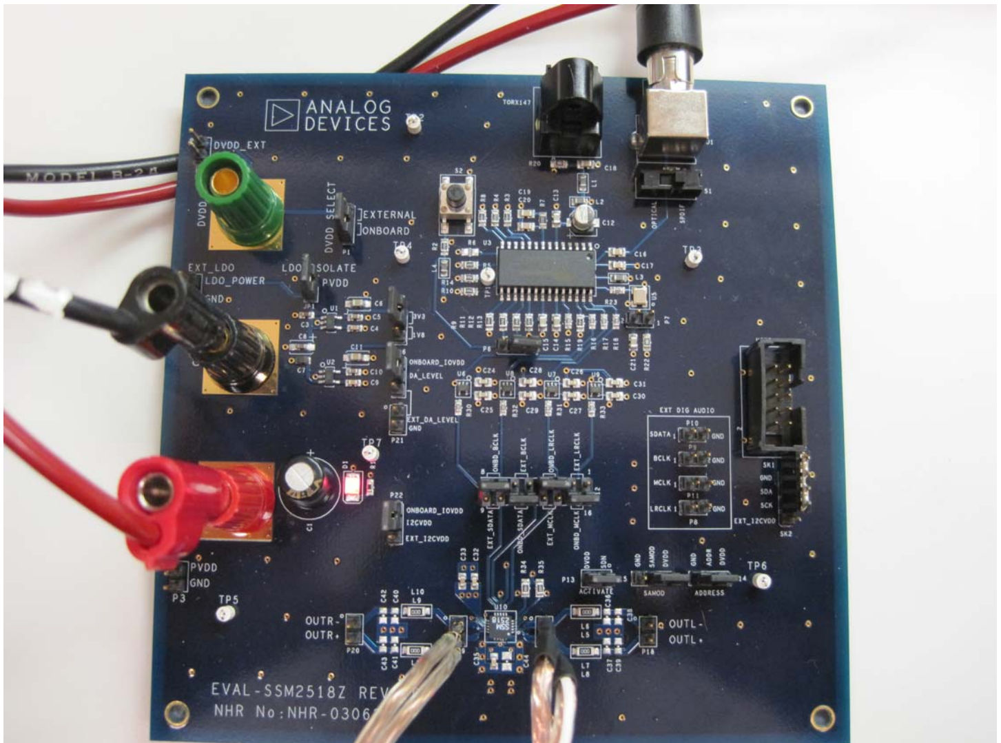
Figure 1: Picture of SSM2518 Evaluation Board (operating in stand-alone mode, without I2C)
