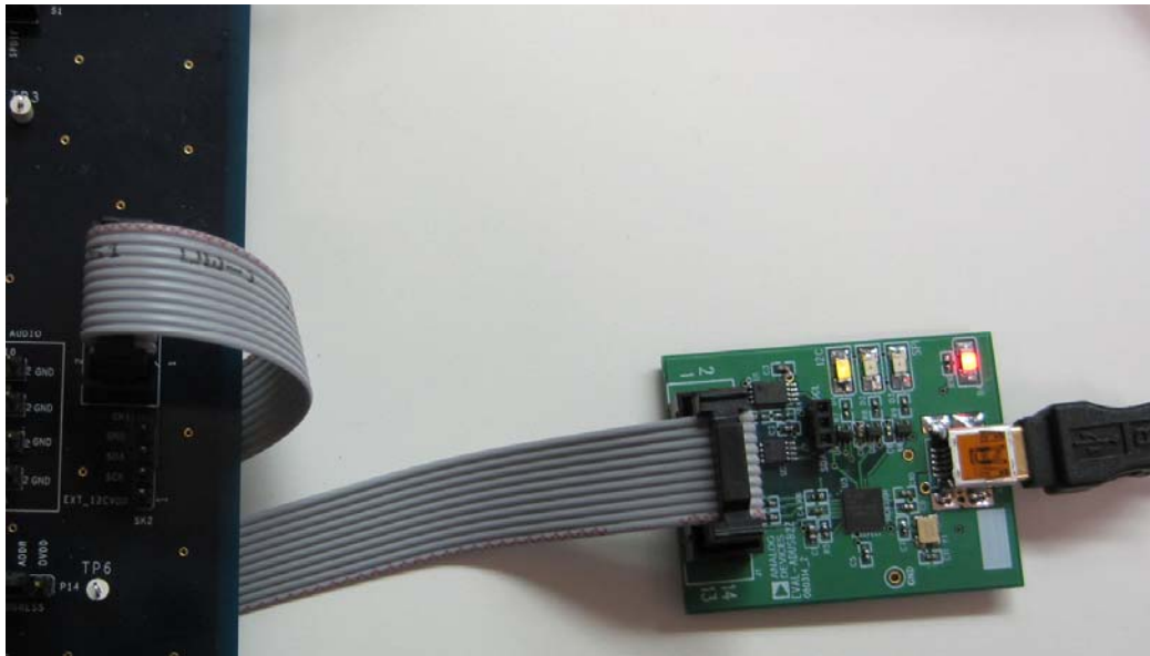
Figure 2: Picture of ADI USB-to-I2C Dongle (ADUSB2)
