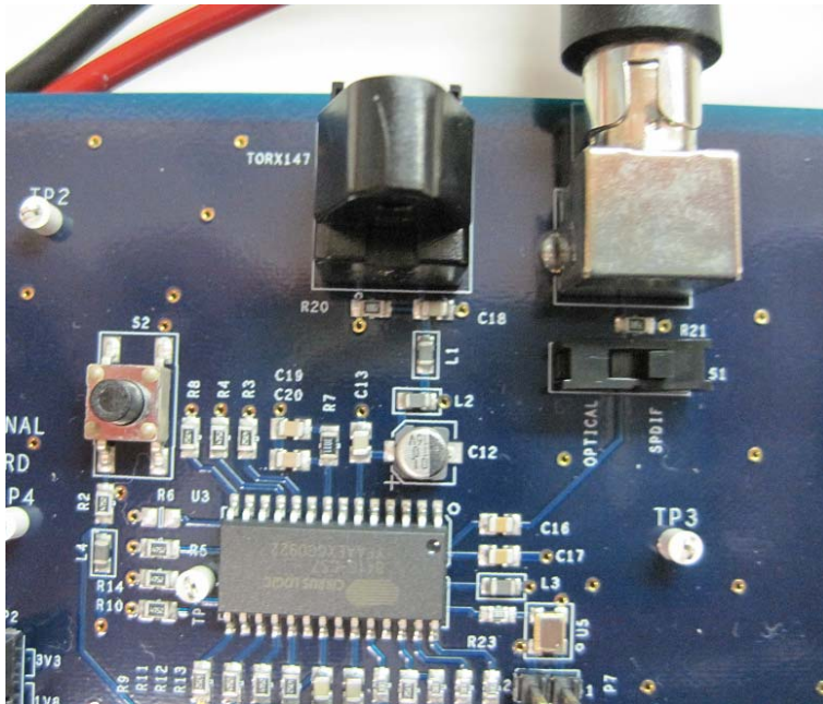
Figure 5: Onboard Digital Audio Source Section
