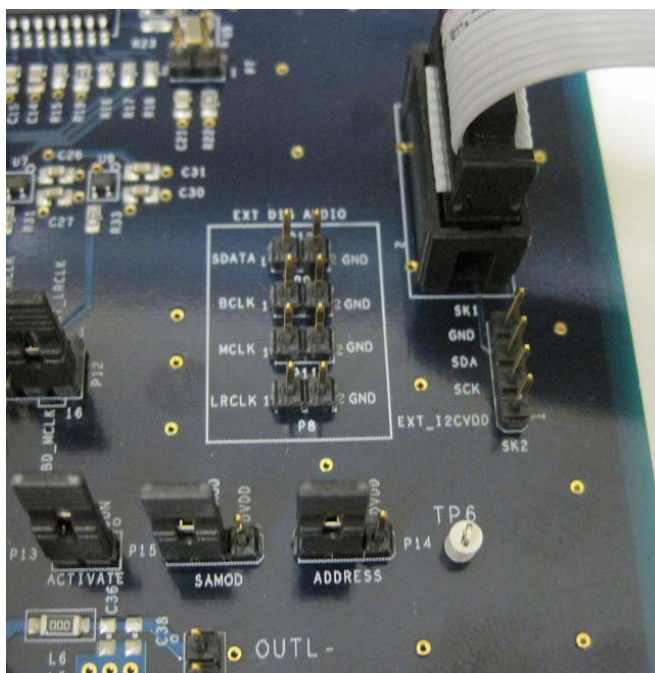
Figure 7: SSM2518 I2C Mode Configuration using ADUSB2 Dongle
